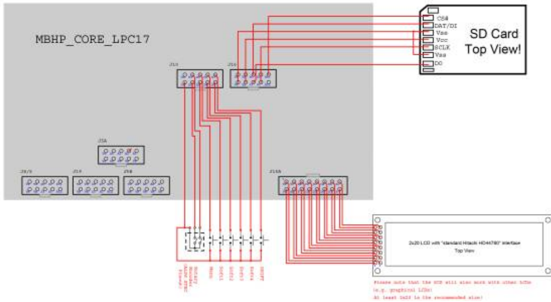
Wiring Diagram for MIDIbox N63 SCS © J. T. Klose 2013-01-02
