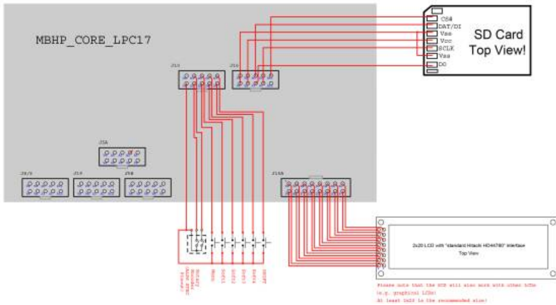
Wiring Diagram for MIDIbox 105 SCS ©21 T. Nöcker 2013-01-02
