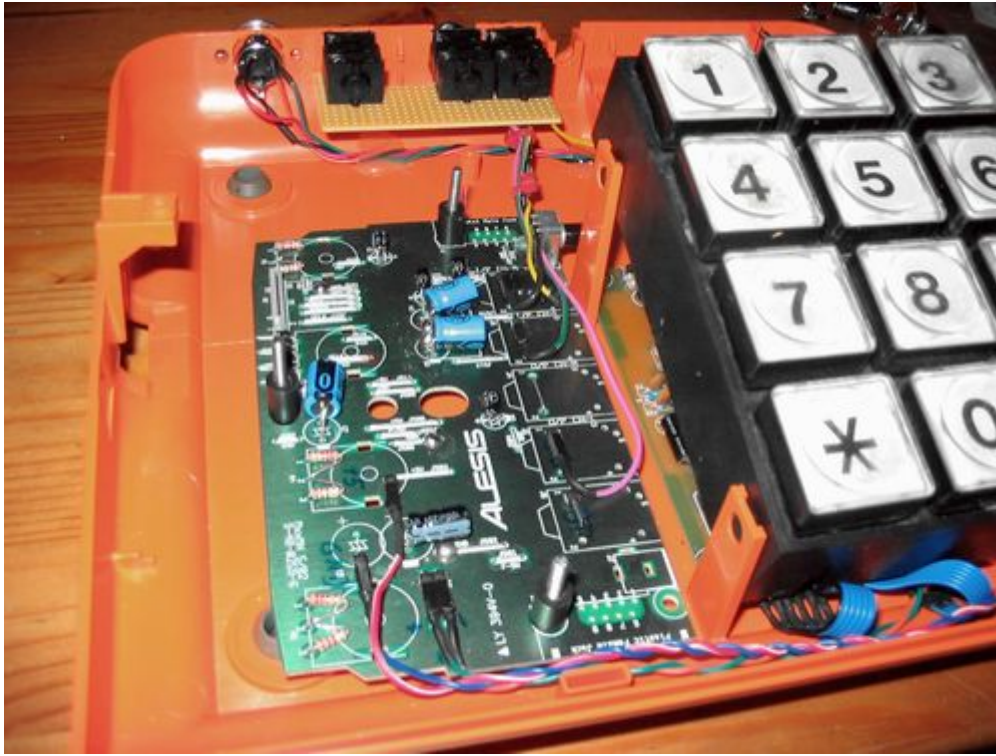
The second board connected. Behind the keypad there's the Sibalance pot.
