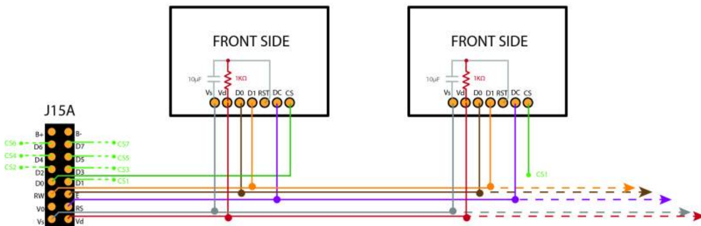
SSD1306 - 128x64px - Pinout Connections
